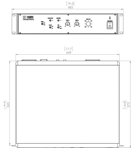
Figure 2 - CCU100 dimensions
