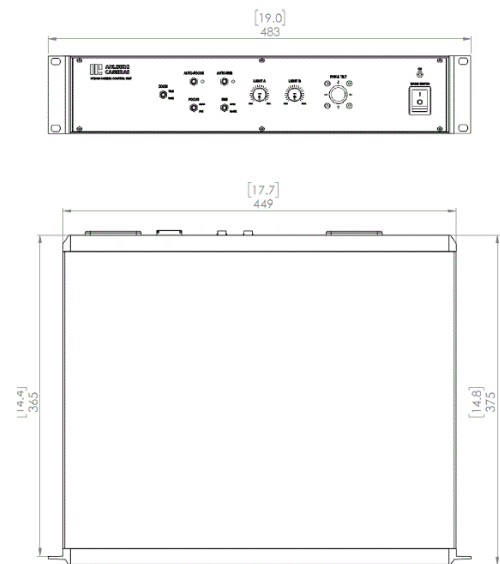
Figure 2 - CCU100 dimensions
